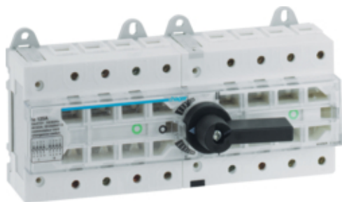
Modular change-over switch 125A
