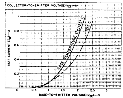
Fig. 11 - Typical input characteristics for 2N3055H, 2N6371, 40251.
