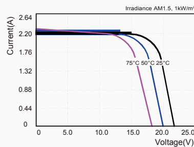
I-V Curves of PV module CL-SM40M at various cell temperatures
