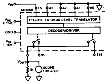
TEST CIRCUIT 2
