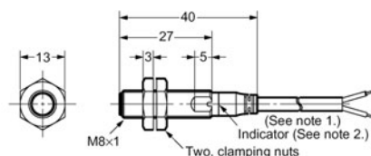
E2A-S08KS02-WP-□□
