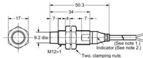
E2A-M12KN08-WP-□□
