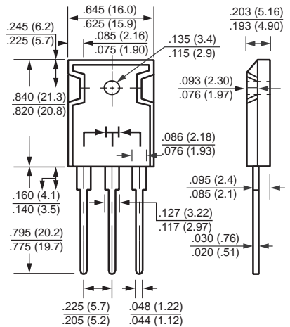
TO-3P
