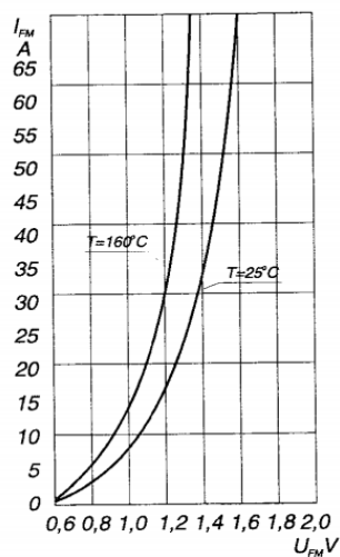
Forward characteristic
