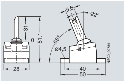
3SE5 000-0AV06 radius actuator approach from right
