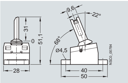
3SE5 000-0AV06 radius actuator approach from right
