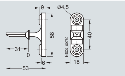
3SE5 000-0AV06 radius actuator approach from right
