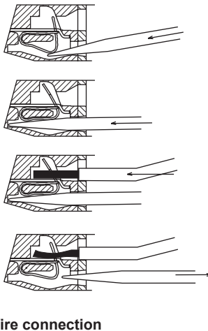
Wire connection
