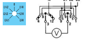
66 - Phase-phase phase-neutral voltmeter changeover / double throw
