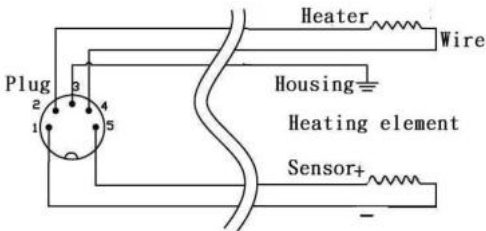
Heating element lead diagram
