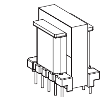
EF 25 reinforced insulation creepage distances: 6mm
