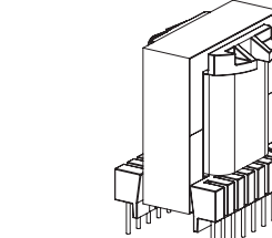
ETD Vertical reinforced insulation creepage distances: 6mm
