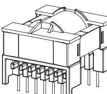
ETD Horizontal reinforced insulation creepage distances: 6mm
