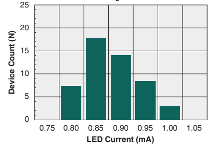
Typical I_F for Switch Dropout (N=50, I_L=300\text{mA} )
