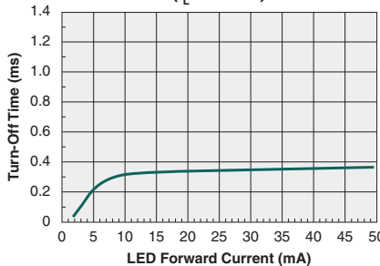
Typical Turn-Off Time vs. LED Forward Current (I L =120mA)
