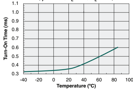
Typical Turn-On Time vs. Temperature ( I_F=10\text{mA} , V_L=10\text{V} , R_L=1\text{k}\Omega )
