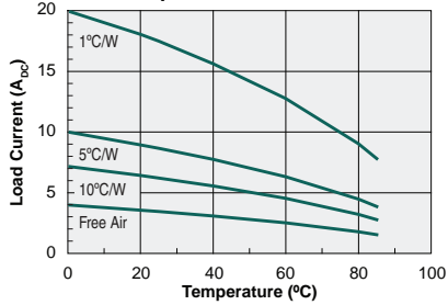
Maximum Load Current vs. Temperature with Heatsink
