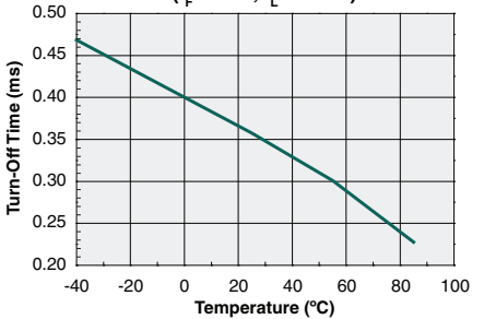
Typical Turn-Off Time vs. Temperature ( I_F=5mA, I_L=80mA )
