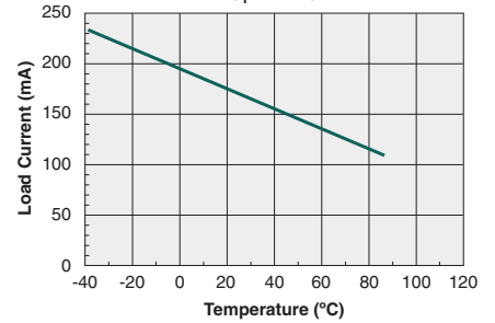
Form-B Maximum Load Current vs. Temperature ( I_F=5mA )
