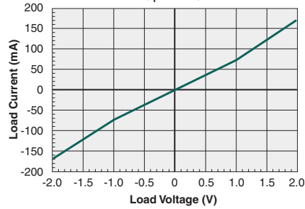
Form-B Typical Load Current vs. Load Voltage ( I_F=5mA )
