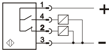
PNP NO+NC ODDxxP311CL
