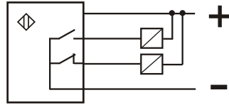
NPN NO+NC ODDxxN31xL
