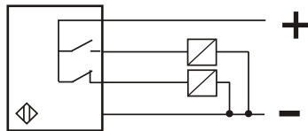
PNP NO+NC ODDxxP31xL
