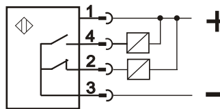
NPN NO+NC ODDxxN311CL
