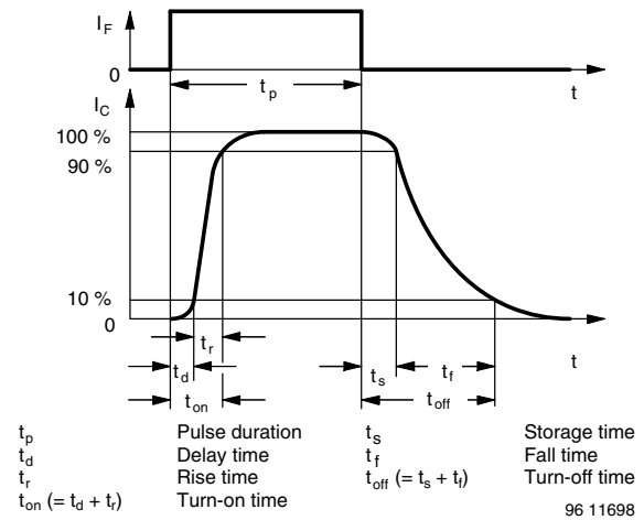
Fig. 4 - Switching Times
