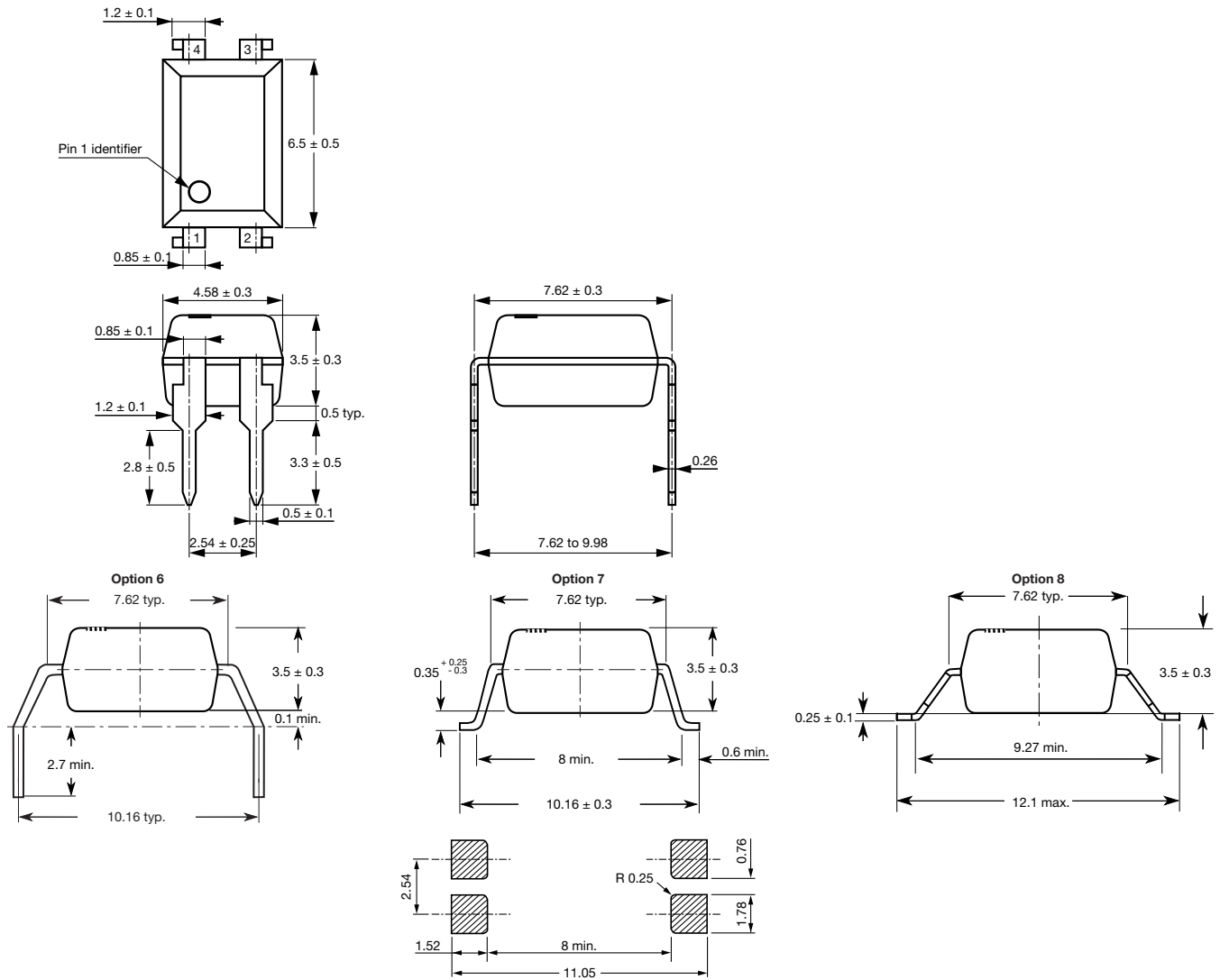
Fig. 17 - Package Drawings
