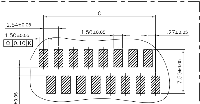
RECOMMENDED PC-BOARD LAYOUT (COMPONENT SIDE OF BOARD SHOWN)
