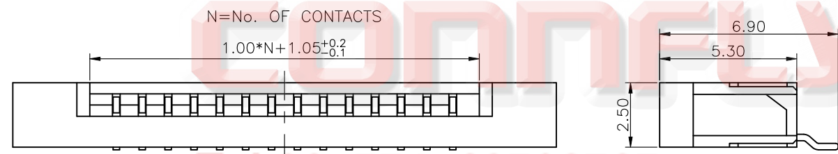
Lower Contact Side
