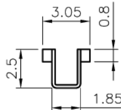
C-C SEC
