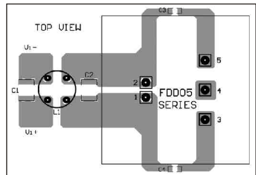
• Recommended EN 55022 Class B filter circuit layout.
