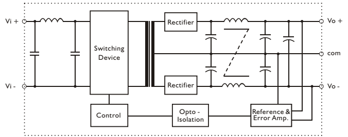
• Block diagram for FDD05 series with dual output
