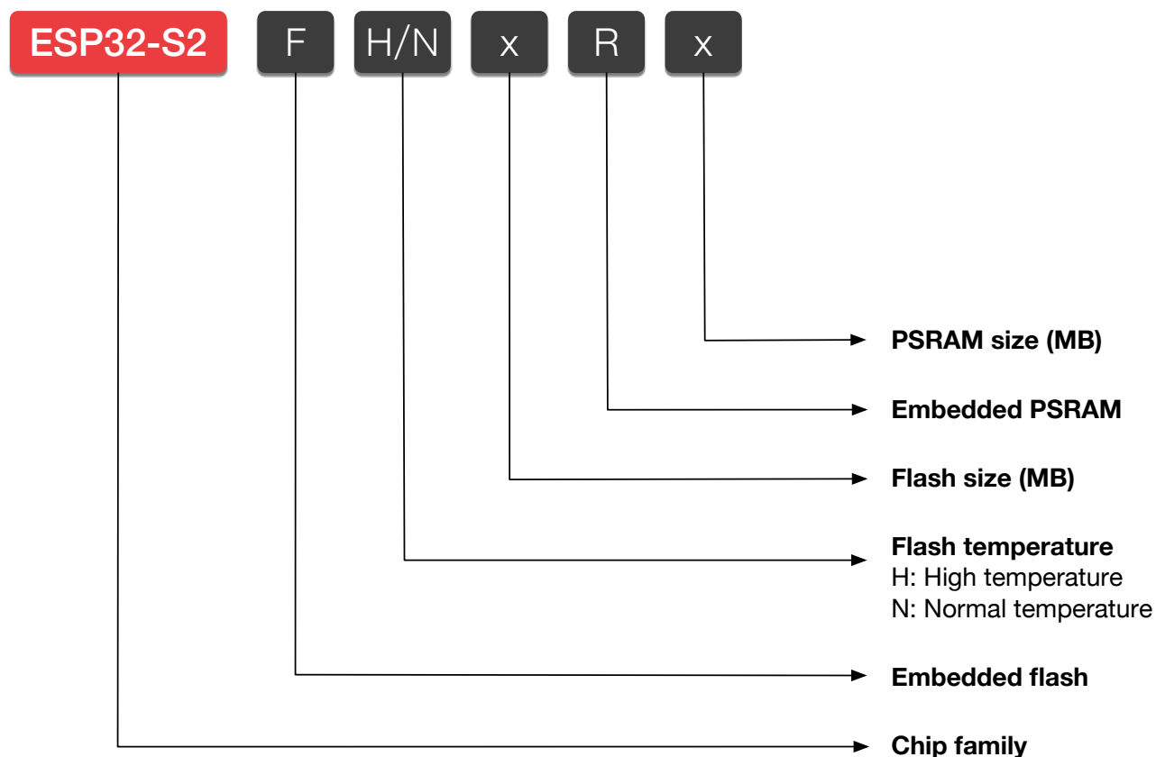
Figure 2: ESP32-S2 Family Nomenclature
