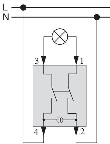
One-way switch 2 pole with indicator light Mxx3x02-0000
