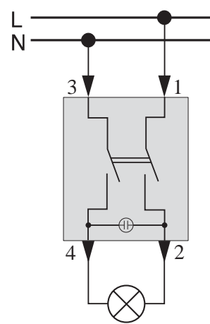
One-way switch 2 pole with indicator light Mxx3x02-0000
