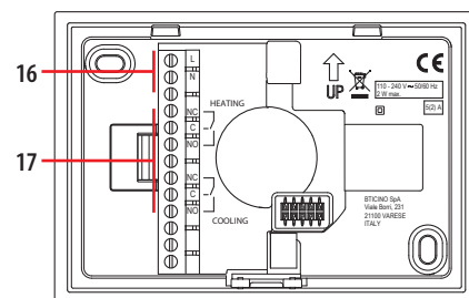
Wall mounted version
