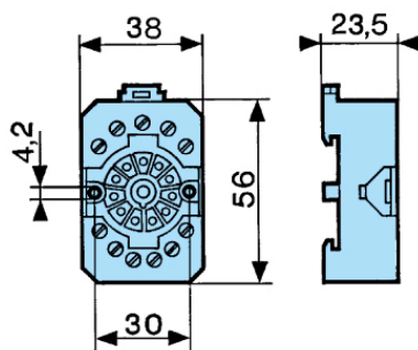
Solder-connected plug: 25622301: 8 pin / 25622076: 11 pin
