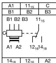
Connection diagram CM-SRS.1, CM-SRS.2
