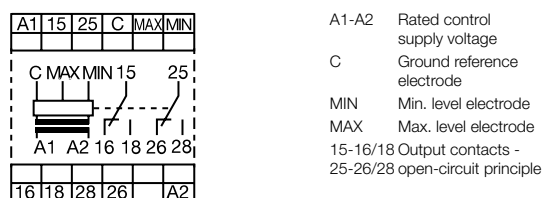
Connection diagram CM-ENN
