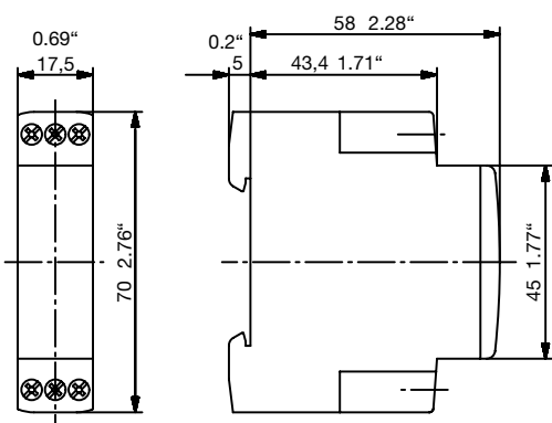
CT-D devices with 1 c/o contact or 2 n/o contacts
