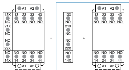
Combination 51 = CAL4-11 + NF(Z)40E
