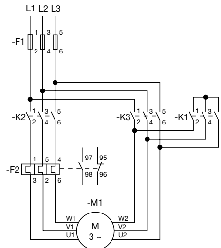
Power circuit diagram
