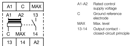
Connection diagram CM-ENN
