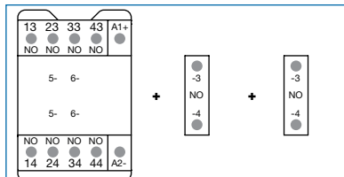
Combination 60E = NS/L40E/S + CA3-10/S + CA3-10/S
