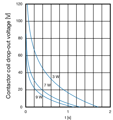
Time delay guideline values 110-127 V AC version
