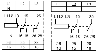
Connection diagram CM-MPS.x3
