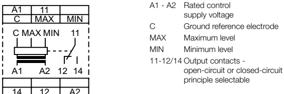
Connection diagram CM-ENS UP/DOWN
