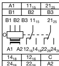
Connection diagram CM-SRS.M
