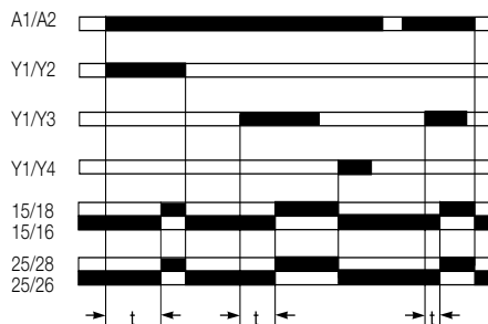
Function diagram CM-KRN
