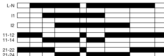
Function diagram CM-SIS
