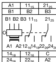
Connection diagram CM-SFS.2
