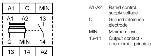
Connection diagram CM-ENE MIN
