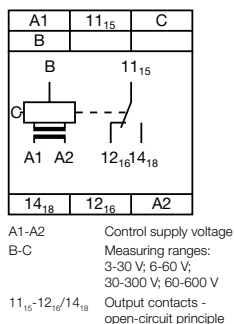
Connection diagram CM-ESS.1, CM-ESS.2
