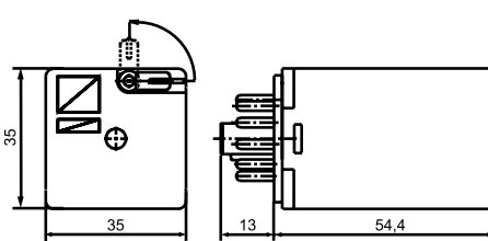
CR-U with 2 c/o contacts
