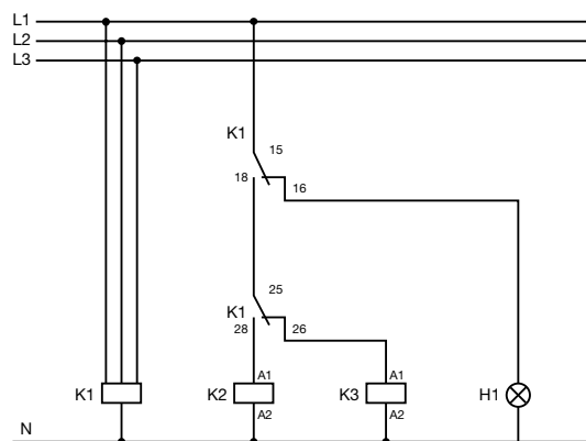
Control circuit diagram (K1 = CM-MPS.xx or CM-MPN.xx)
