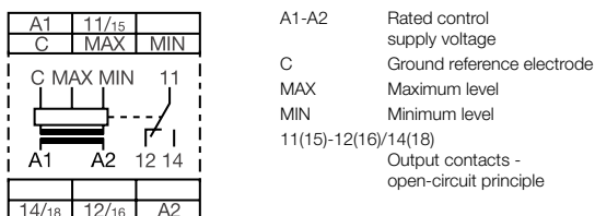
Connection diagram CM-ENS
