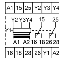
Connection diagram CM-KRN
