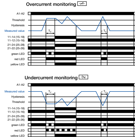
Function diagrams CM-SRS.2
