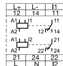
Connection diagram CM-SIS
