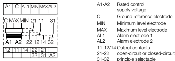
Connection diagram CM-ENN UP/DOWN
