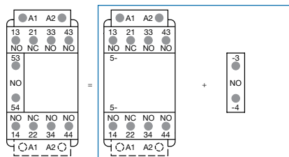
Combination 41 = NF(Z)31E + CA4-10
