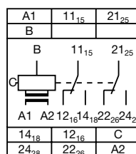
Connection diagram CM-ESS.M
