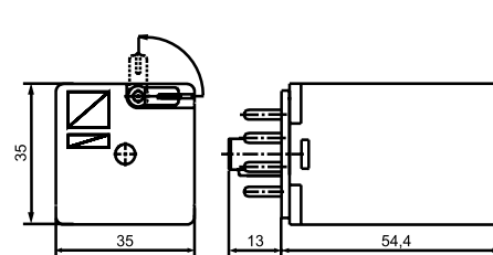
CR-U with 2 c/o contacts
