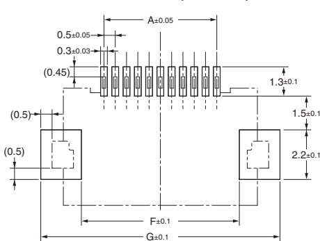
PCB Dimensions (TOP VIEW)
