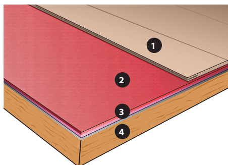
Fig. 17. Floor heating with DEVIDry™ on existing wooden subfloor
