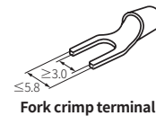
Fork crimp terminal
