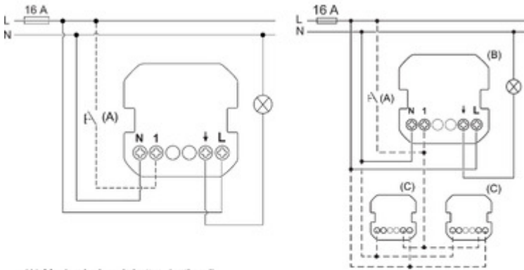
(A) Mechanical push-button (optional) (B) Primary motion sensor (C) Secondary motion sensor
