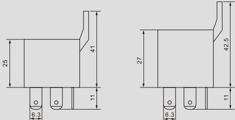
AS403 Outline dimension
