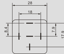
AS403 Mounting holes (Bottom view)
