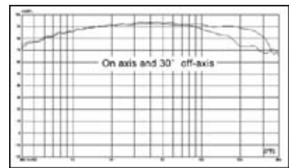
Frequency Response (Magnify)
