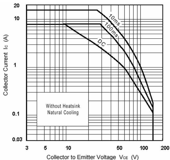
Fig.4 Safe Operating Area (Single Pulse)
