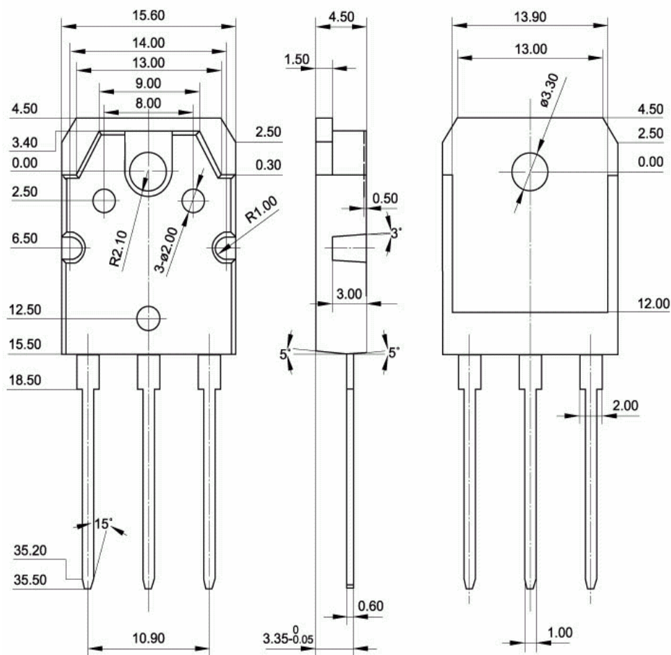
Fig.2 Outline dimensions
