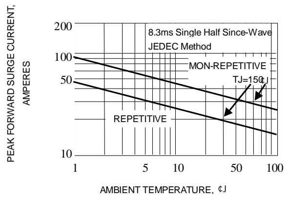
Fig. 2-MAXIMUM PEAK FORWARD SURGE CURRENT
