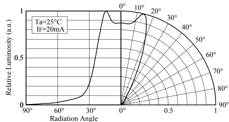
■ Directivity (NSPW510B(S))
