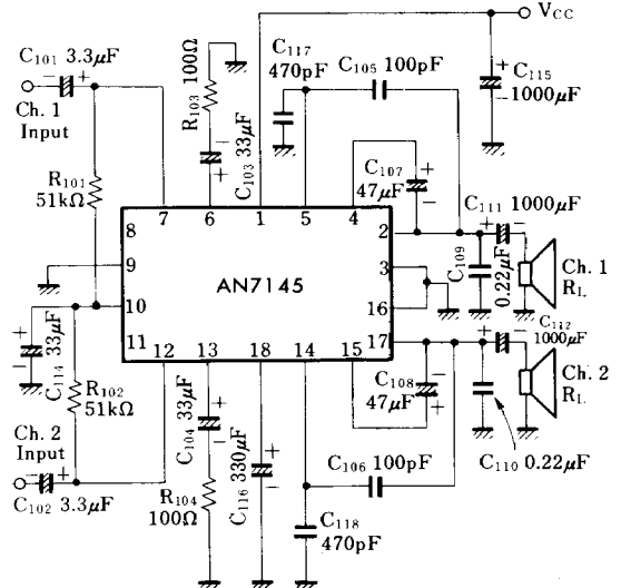
Test Circuit 2 (Dual Circuit)
