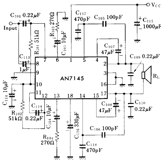
Test Circuit 1 (BTL Circuit)
