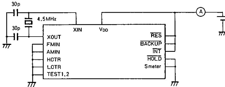
Fig. 1 I_{DD}(2) measurement circuit in the HOLD mode
