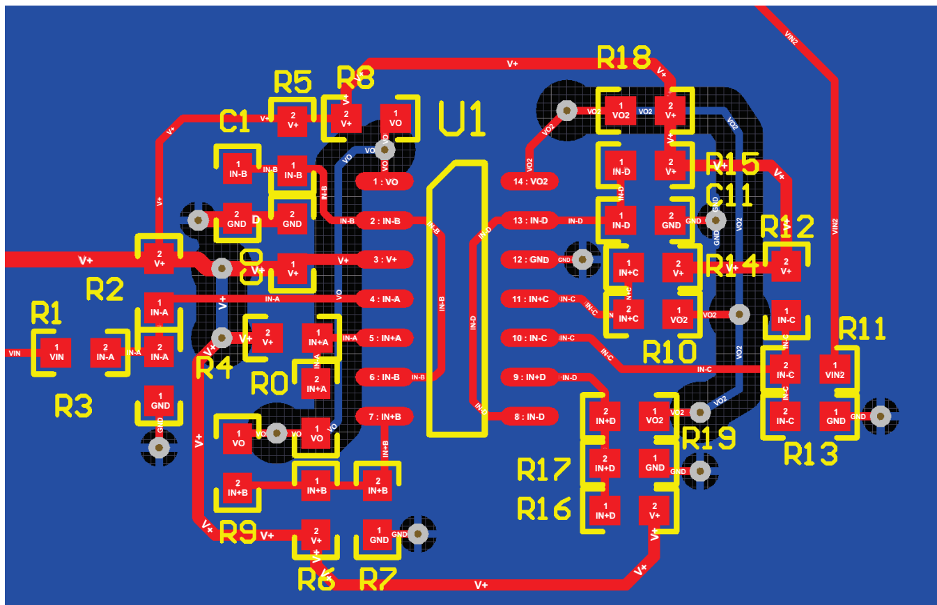
Figure 43. Layout Example
