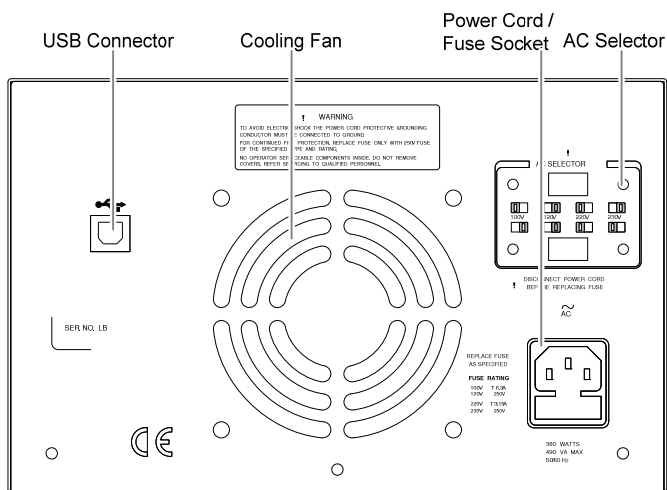
USB Connector
